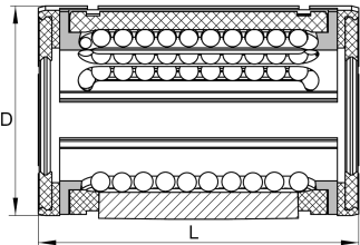
KS16, 20 KSO16, 20
